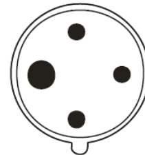
Front View of Plug
