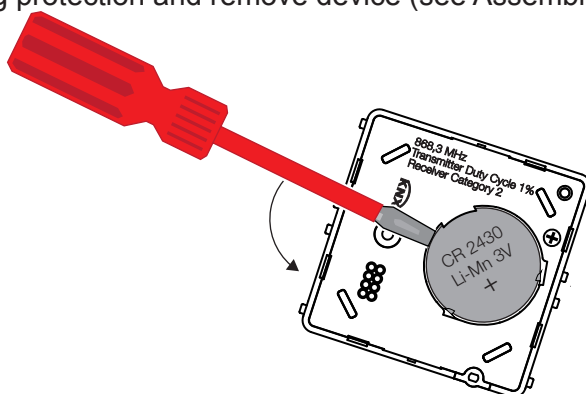
Figure 4: Remove battery
