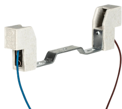
141213 Lampholder R7s 118MM 6A 250V T250°C 250mm
